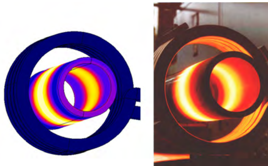
Simulation du processus de chauffage par induction. Altair Flux™ ©1983-2021, held by Altair Engineering Inc.
